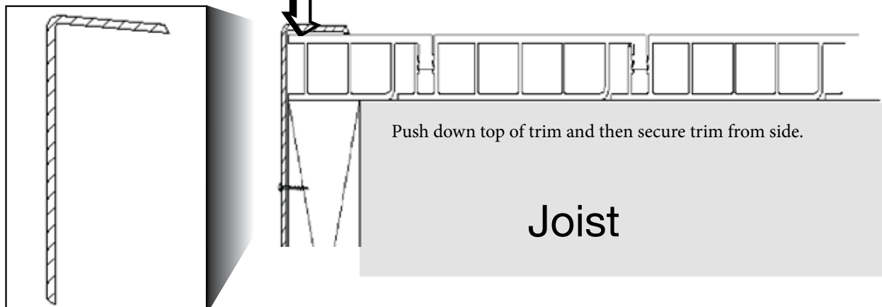
(Figure 8 - Fascia trim detail.)
