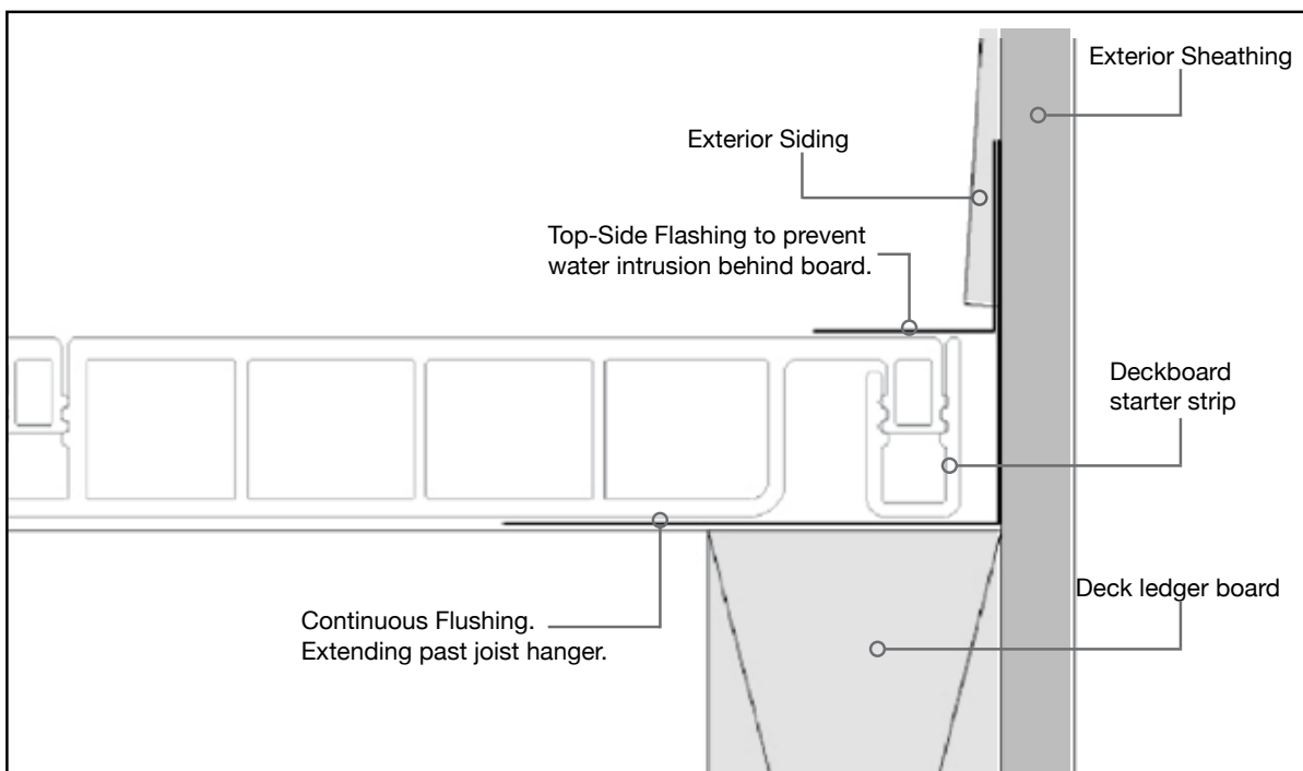
(Figure 1 - Flashing detail)
